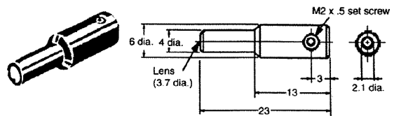
E39-F3A Reflective unit lens (Allen wrench included)
