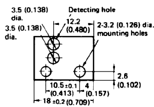
E39-F5 Side-view diffuse reflective conversion kit
