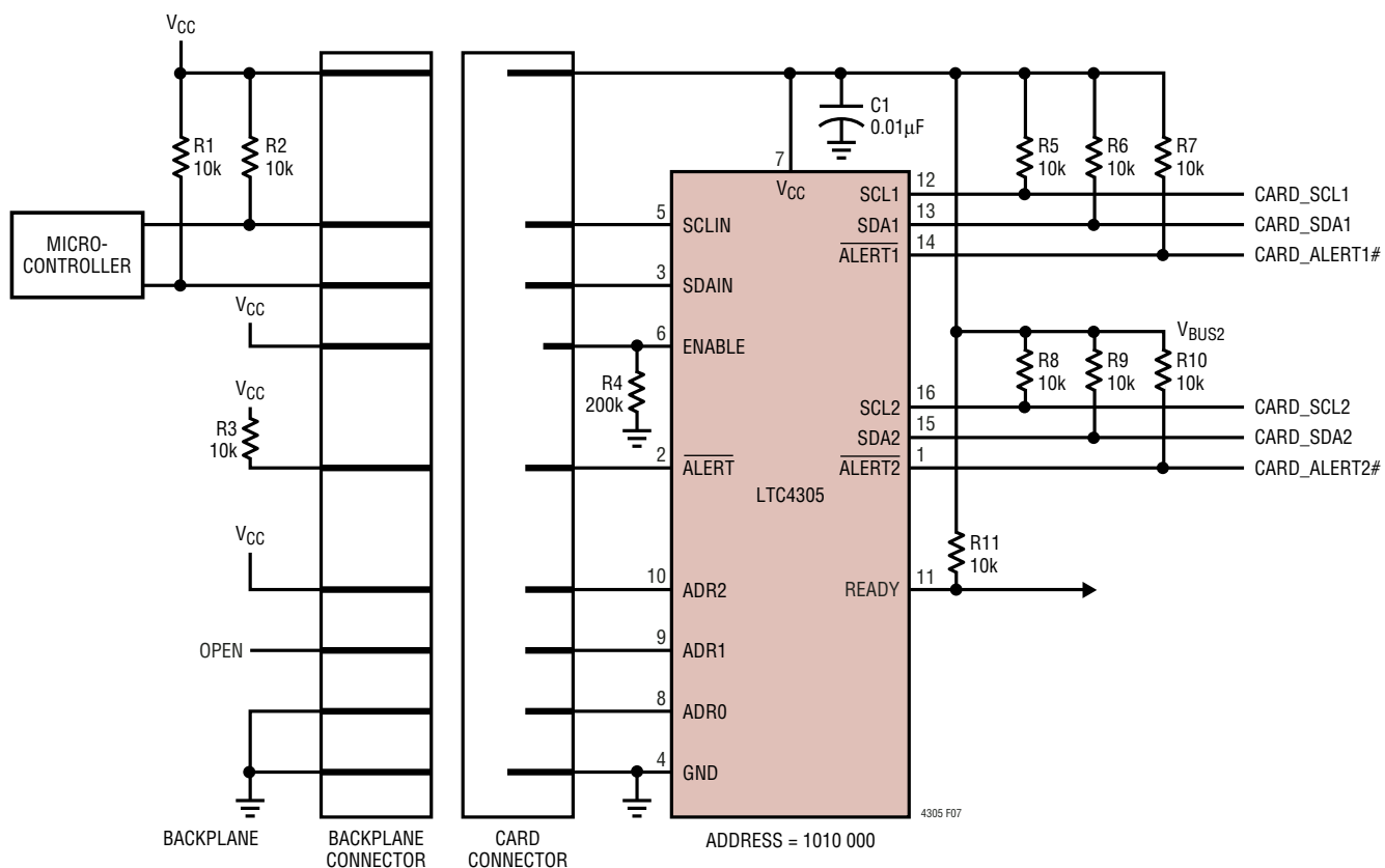
Figure 7. Hot-Swapping Application
