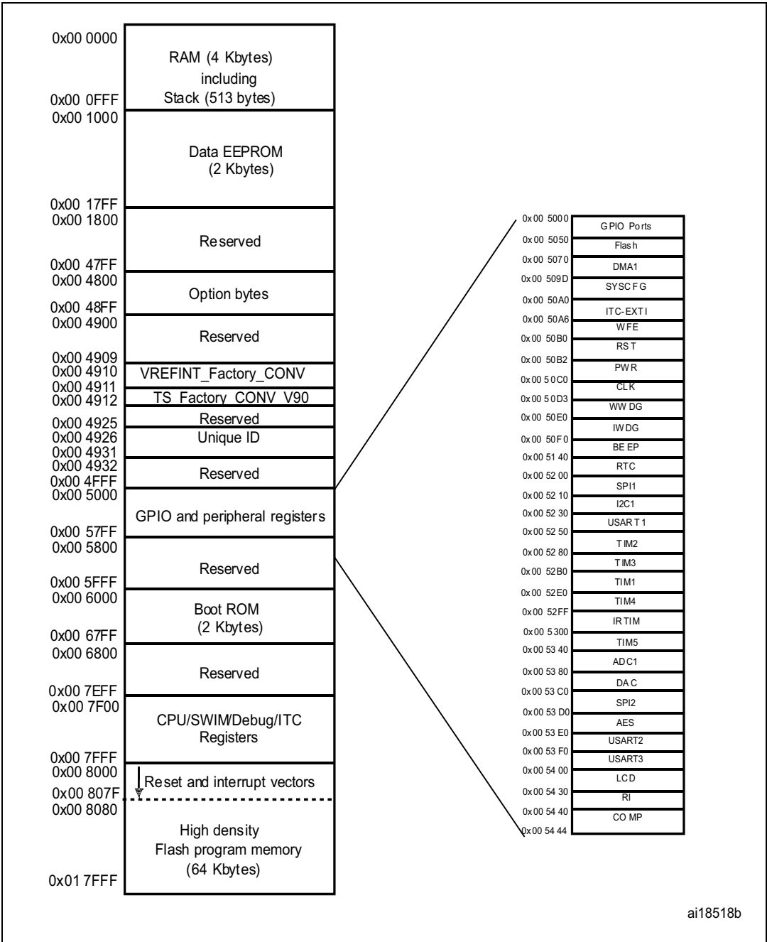
Figure 5. Memory map
