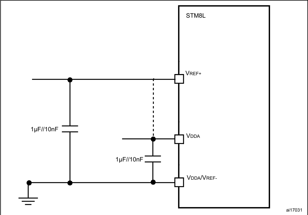
Figure 40. Power supply and reference decoupling ( V_{REF+} not connected to V_{DDA} )
