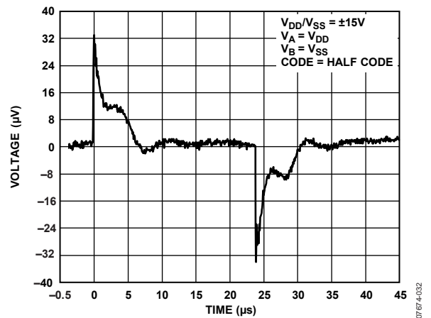
Figure 53. Digital Feedthrough
