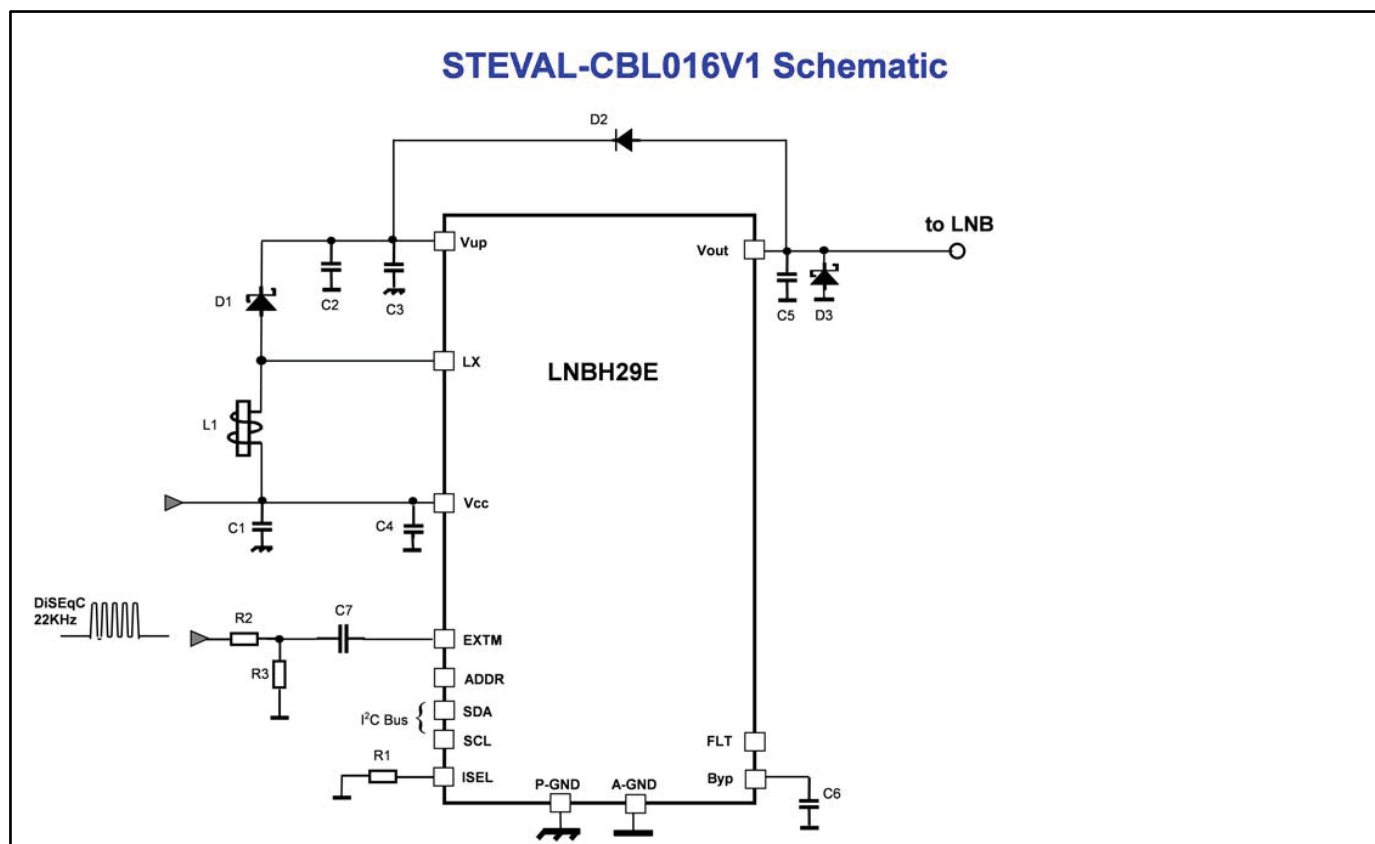
Figure 1: STEVAL-CBL016V1 schematic
