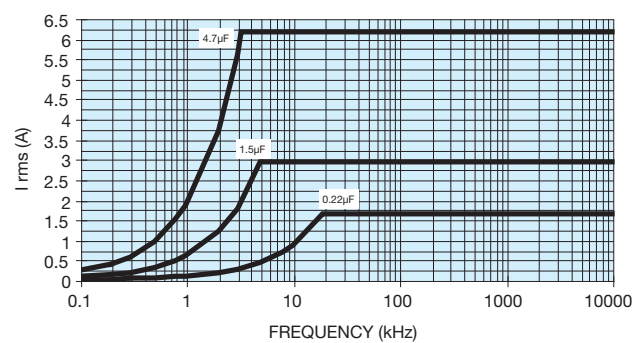
100 Vdc / 63 Vac
