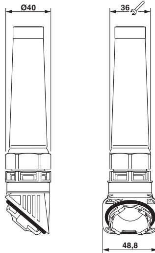
Dimensional drawing
