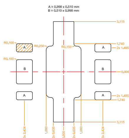
PCB METAL LAND PATTERN
