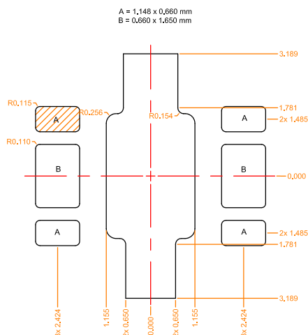
PCB SOLDER MASK PATTERN
