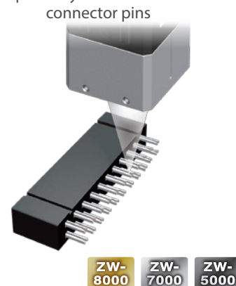
Coplanarity measurement of connector pins
