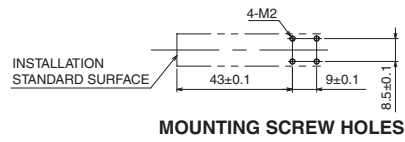
MOUNTING SCREW HOLES
