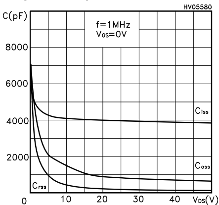
Figure 9. Capacitance variations
