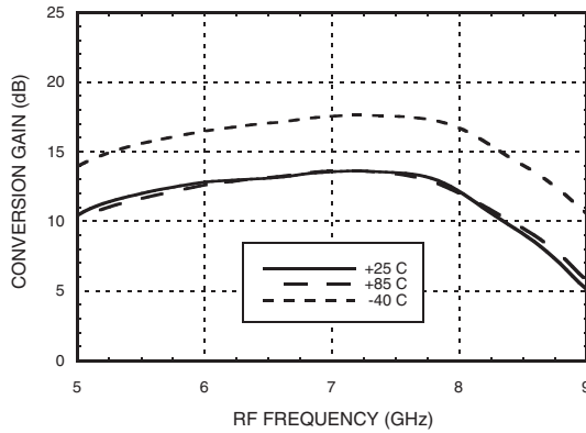
Conversion Gain, LSB vs. Temperature
