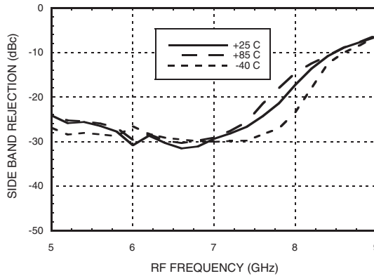
Sideband Rejection vs. Temperature
