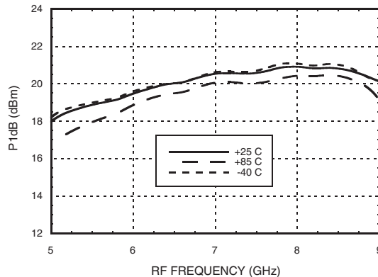
Output P1dB, LSB vs. Temperature
