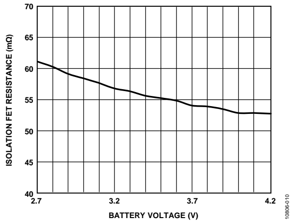
Figure 10. Ideal Diode R_{ON} vs. Battery Voltage, I_{ISO\_Sx} = 500 mA, V_{INx} Open
