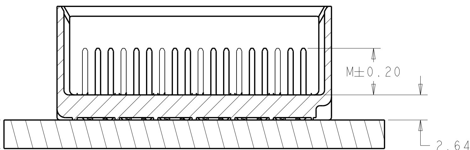
SECTION Z-Z
