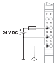
Connection diagram
