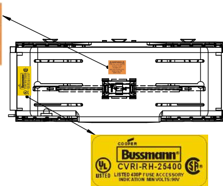
RM25400-1CR WITH CVRI-RH-25400 INSTALLED
