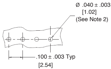
Recommended Mounting Hole Pattern
