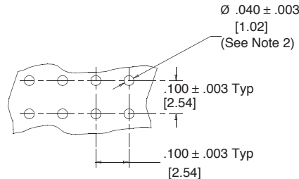
Recommended Mounting Hole Pattern
