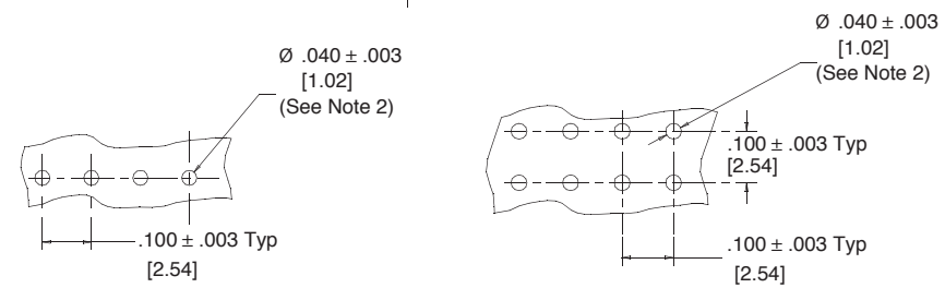
Recommended Mounting Hole Pattern
