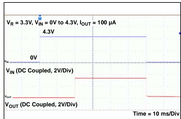
FIGURE 2-30: Start-up from V_{IN} ( V_R = 3.3\text{V} ).
