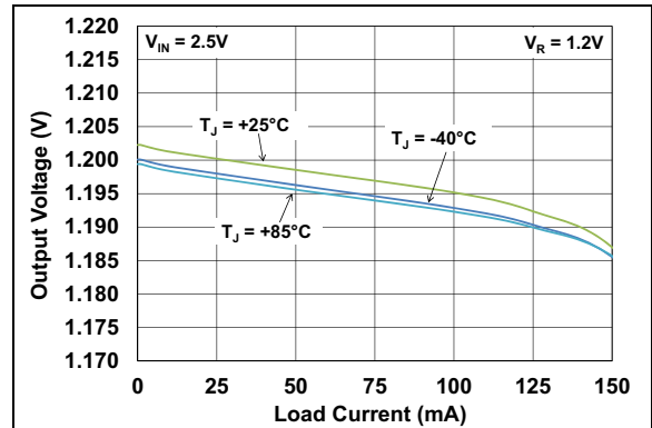
FIGURE 2-5: Output Voltage vs. Load Current ( V_R = 1.2\text{V} ).
