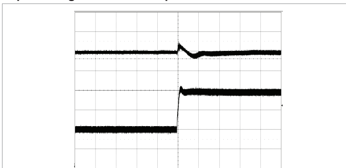
Output voltage response to input voltage transient at: T_{P1}, T_{P3} = +25^\circ\text{C}, V_i = 36-75\text{ V}, I_o = 17\text{ A} resistive load, C_o = 3.5\text{ mF} Top trace: output voltage (2 V/div.). Bottom trace: input voltage (20 V/div.). Time scale: (0.5 ms/div.).
