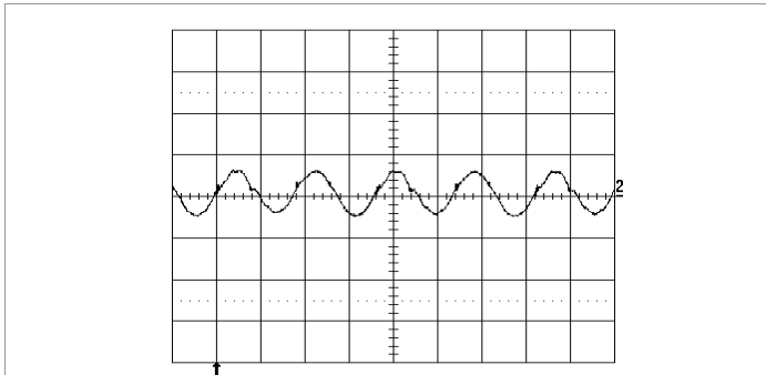
Output voltage ripple at: T_{P1}, T_{P3} = +25^\circ\text{C}, V_i = 53\text{ V}, I_o = 35\text{ A} resistive load. Trace: output voltage (50 mV/div.). Time scale: (2 μs/div.).
