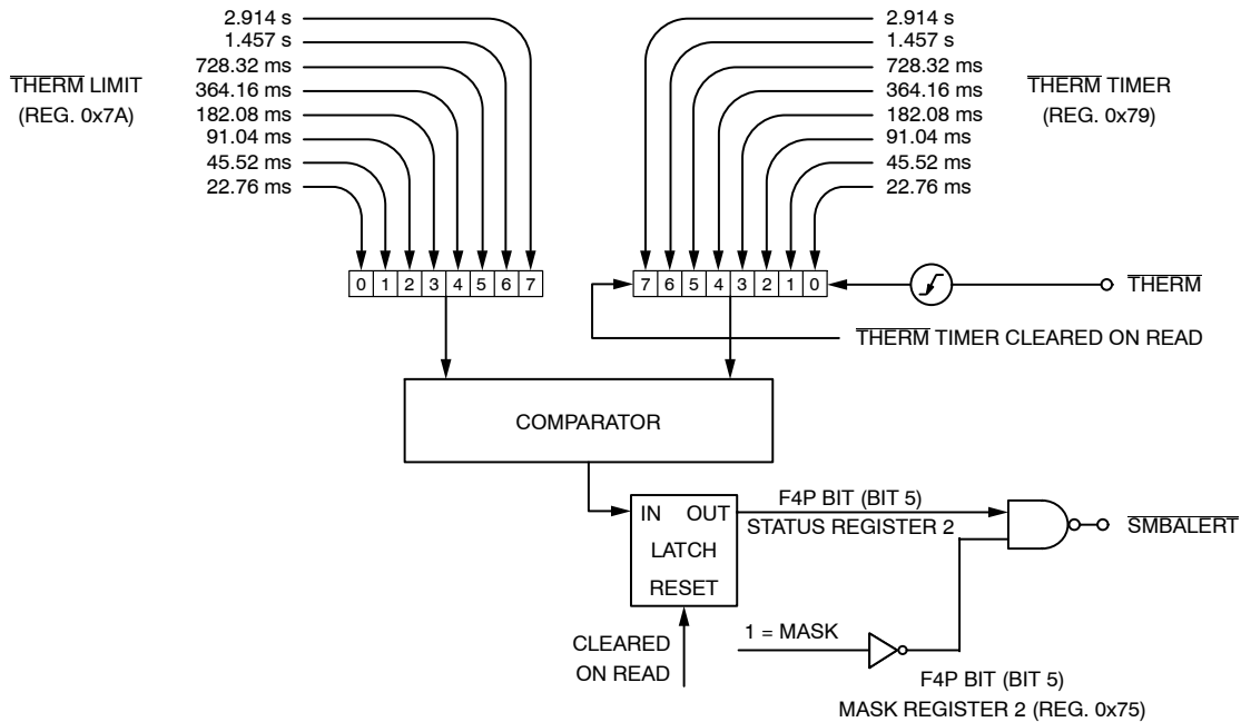
Figure 33. Functional Block Diagram of \overline{THERM} Monitoring Circuitry
