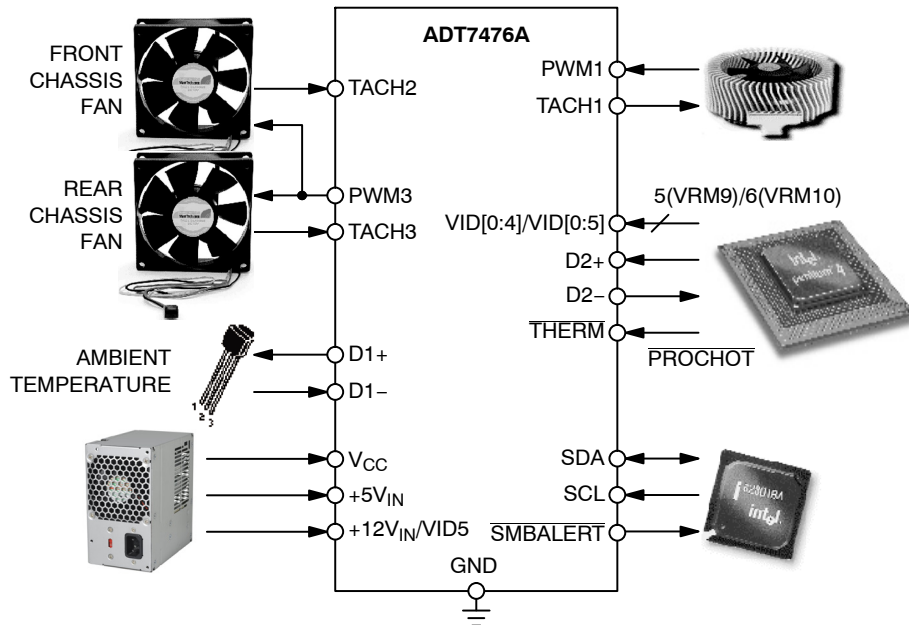
Figure 13. ADT7476A Configuration
