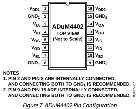
Figure 7. ADuM4402 Pin Configuration
