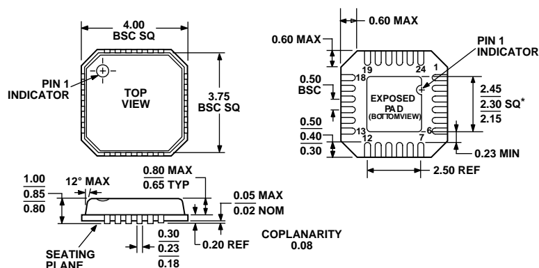
Figure 47. 24-Lead Lead Frame Chip Scale Package [LFCSP] 4 × 4 mm Body (CP-24-2) Dimensions shown in millimeters
