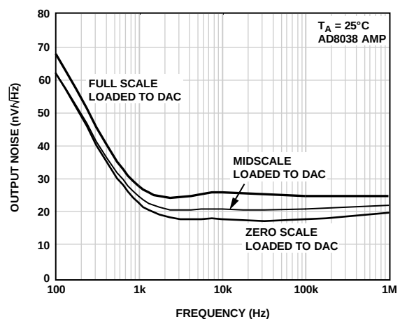
Figure 36. Output Noise Spectral Density
