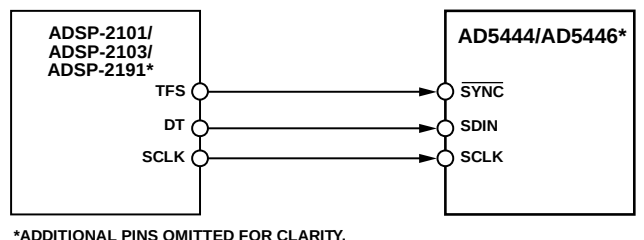
Figure 47. ADSP-2101/ADSP-2103/ADSP-2191 SPORT to AD5444/AD5446 Interface
