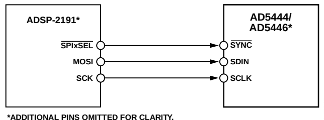
Figure 46. ADSP-2191M SPI to AD5444/AD5446 Interface
