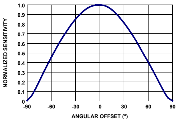
FIGURE 8. ANGULAR SENSITIVITY
