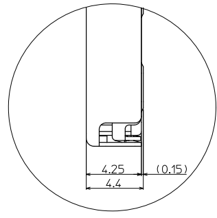
DETAIL B (5:1)
