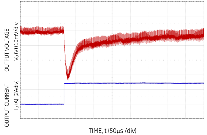
Figure 10. Transient Response to Dynamic Load Change from 50% to 100% at 12Vin, Cout-1x330μF, 4x100μF, Ctune-4.7nF, Rtune-500
