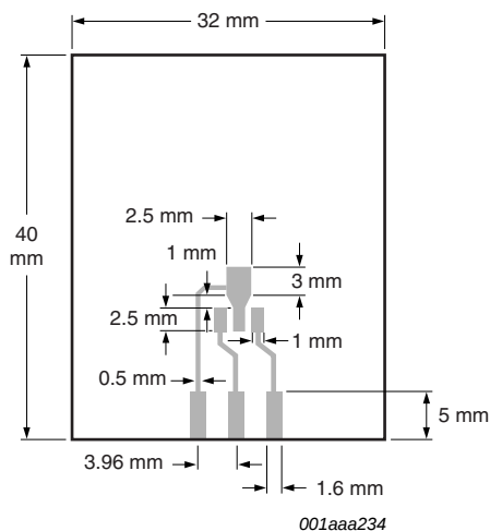
PCB thickness: FR4 PCB = 1.6 mm ceramic PCB = 0.635 mm Fig 18. FR4 PCB, standard footprint; ceramic PCB, Al_2O_3 , standard footprint
