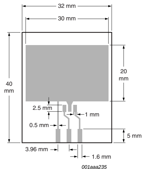
PCB thickness = 1.6 mm Fig 19. FR4 PCB, mounting pad for collector 6 cm 2
