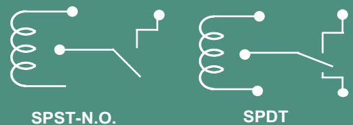
WIRING DIAGRAMS (VIEWED FROM PIN END)
