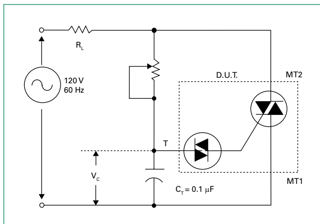
Figure 9: Test Circuit
