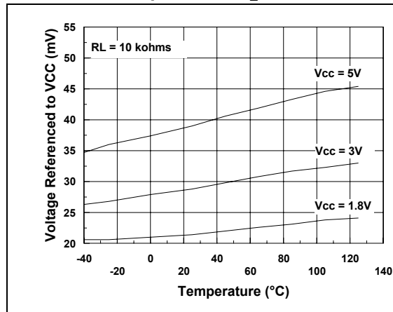
Figure 17. High level output voltage vs. temperature, R_L = 10\text{ k}\Omega
