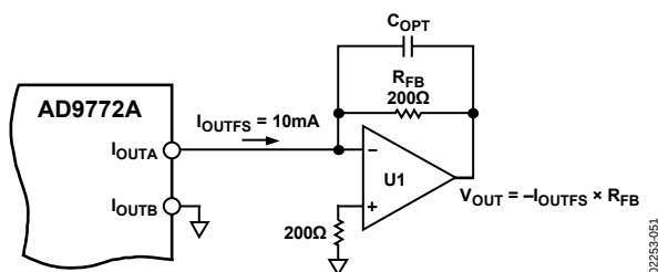
Figure 51. Unipolar Buffered Voltage Output
