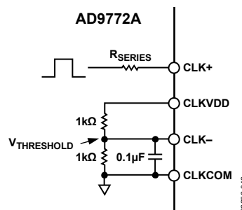
Figure 43. Single-Ended Clock Interface
