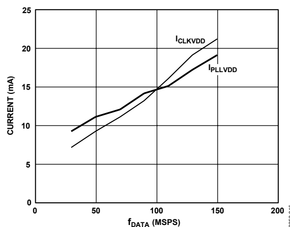
Figure 46. I_{PLLVD} and I_{CLKVD} vs. f_{DATA}
