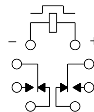
TERMINAL VIEW
