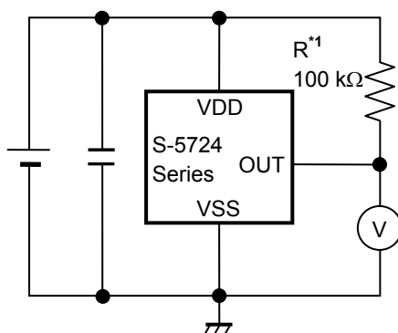
Figure 10 Test Circuit 3
