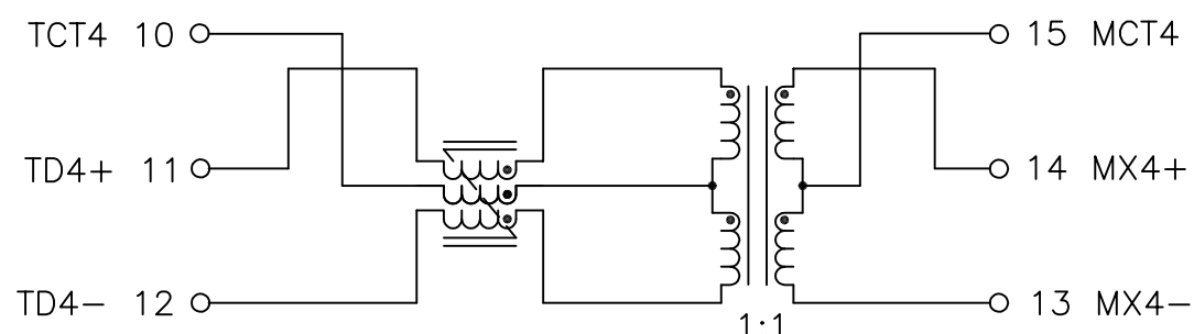
SCHEMATIC
