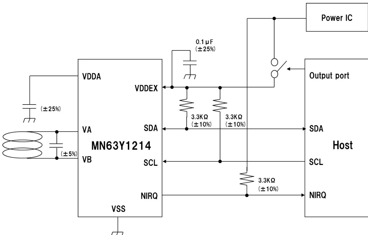
Figure 2-3 Connection Example
