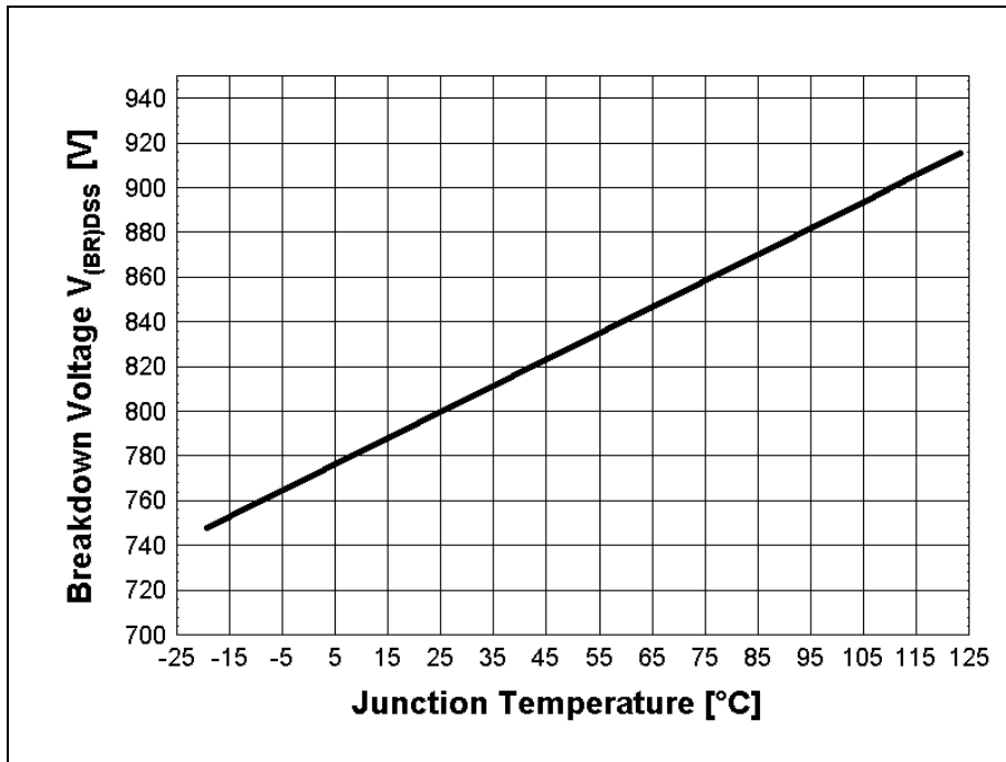
Figure 9 Drain-source breakdown voltage; V_{BR(DSS)} = f(T_J), I_D = 0.25mA
