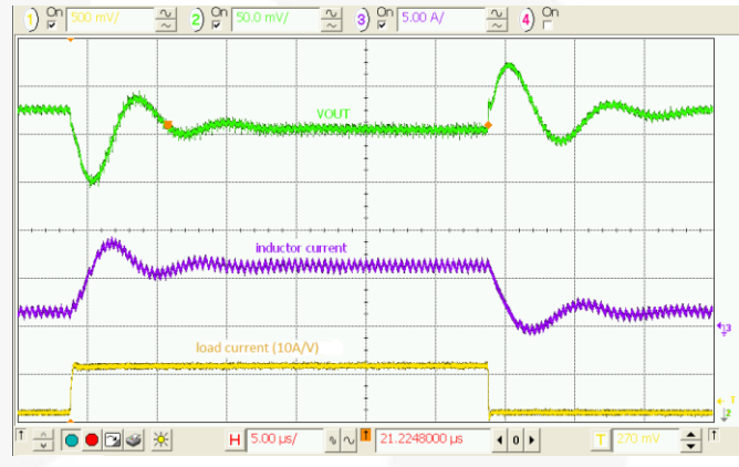
Figure 28. Load Transient, 3.6 V IN , 1.2 V OUT , 1.5-6 A, 100 ns Edge, C OUT =4x22 μF
