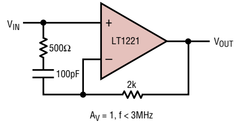
Lag Compensation
