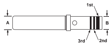
M39029/22 Contact Dimensions
