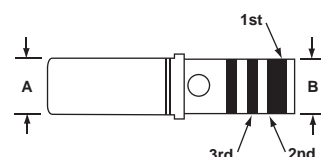
M39029/22 Contact Dimensions
