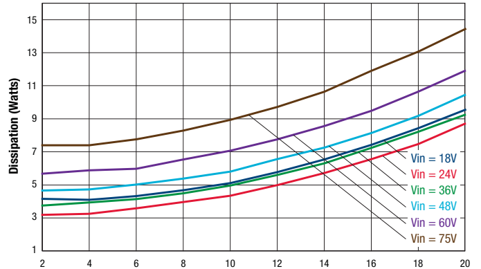
Power Dissipation vs. Line and Load
