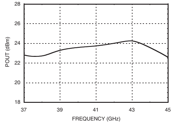
Fixtured P1dB vs. Frequency
