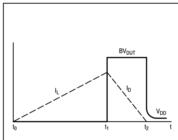
Figure 14. Current-Voltage Waveforms
