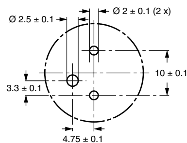
Fig.3 Mounting hole diagram
