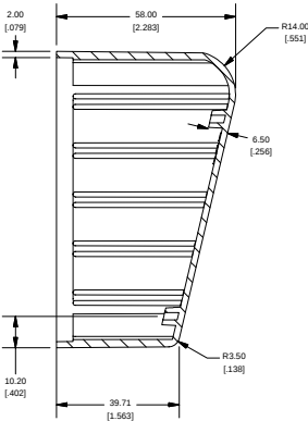
SECTION A-A SCALE 3 / 4
