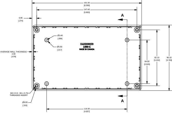
ENCLOSURE
