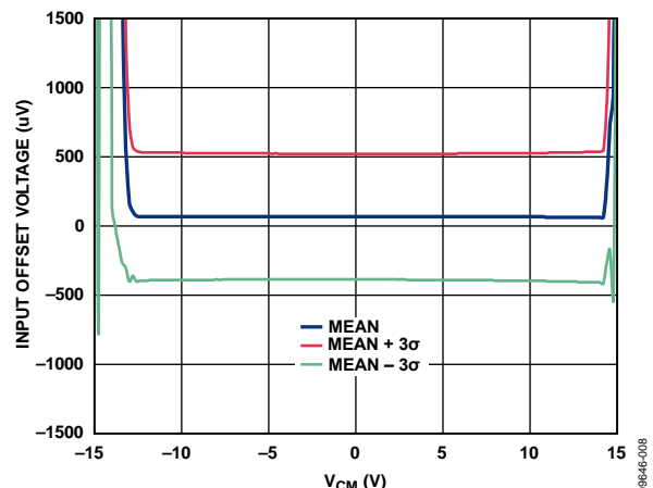
Figure 13. Input Offset Voltage vs. Input Common-Mode Voltage ( V_{CM} ), V_{SY} = \pm 15 V, R_L = \infty
