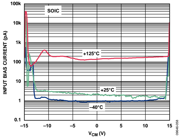
Figure 18. Input Bias Current vs. Common-Mode Input Voltage ( V_{CM} ), V_{SY} = \pm 15V, R_L = \infty
