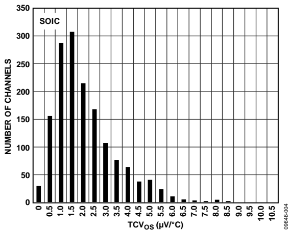
Figure 9. Input Offset Voltage Drift ( TCV_{OS} ) Distribution, V_{SY} = \pm 5 V
