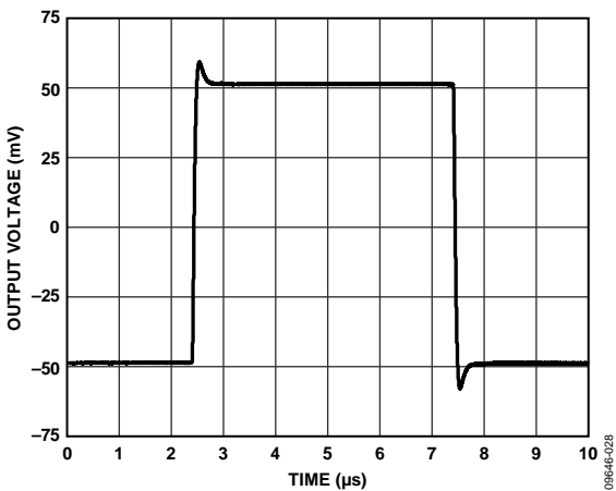
Figure 34. Small Signal Transient Response, V_{SY} = \pm 5 V , A_V = +1 , R_L = 2 k\Omega , C_L = 100 pF
