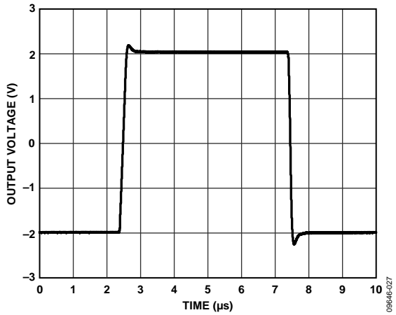
Figure 33. Large Signal Transient Response, V_{SY} = \pm 5 V , A_V = +1 , R_L = 2 k\Omega , C_L = 100 pF
