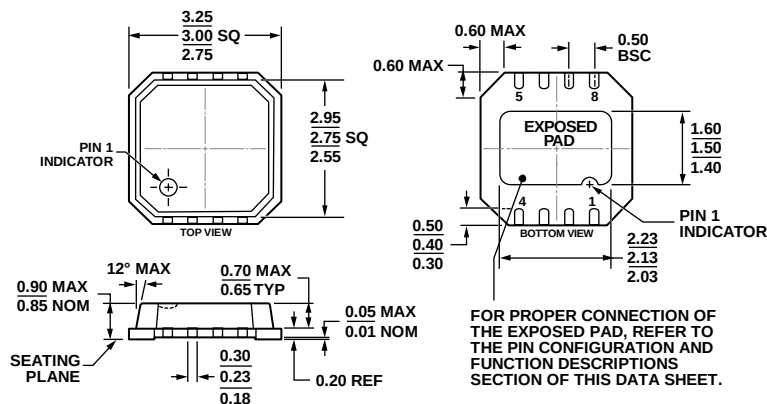
Figure 62. 8-Lead Lead Frame Chip Scale Package [LFCSP_VD] 3 mm × 3 mm Body, Very Thin, Dual Lead (CP-8-9)
