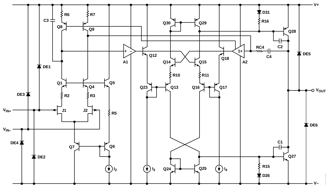
Figure 56. Simplified Schematic
