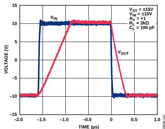
Figure 55. Positive and Negative Slew Rate ( V_{SY} = \pm 15\text{ V} , A_V = +1 , R_L = 2\text{ k}\Omega )
