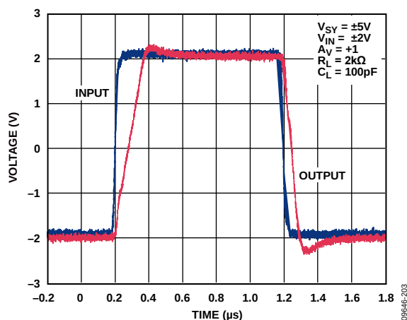
Figure 54. Positive and Negative Slew Rate ( V_{SY} = \pm 5\text{ V} , A_V = +1 , R_L = 2\text{ k}\Omega )
